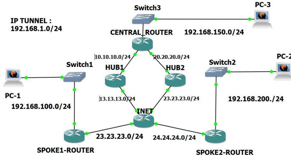
Gambar 1. Topologi DMVPN
