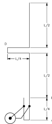
Gambar 2. Antena Super J-Pole
